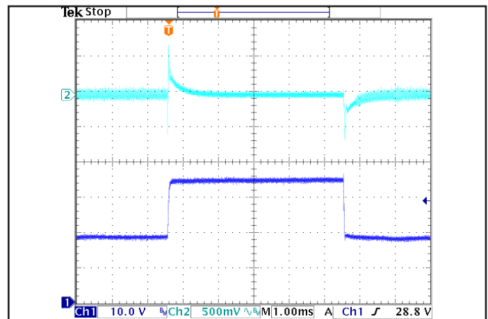
Figure 6: Output voltage response to step-change in input voltage (1000 V/ms). Load cap: 1 μF ceramic capacitor. Ch 1: Vin, Ch 2: Vout.
